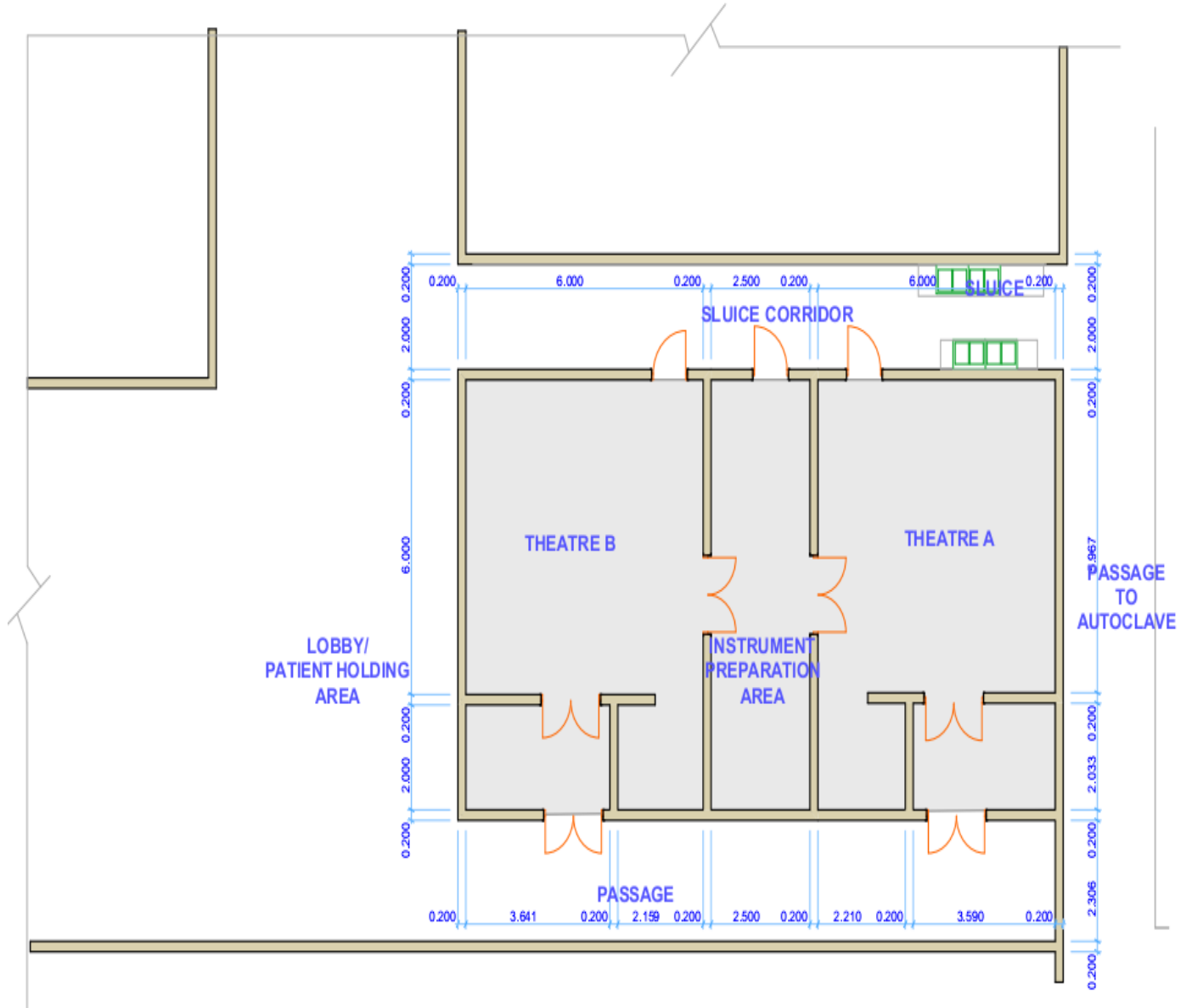
MTRH PART THEATRE LAYOUT
